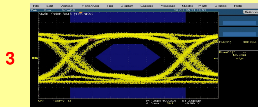
Eye Pattern with Mask: 1000B - SX/LX (1.25Gb/s) at location 3
