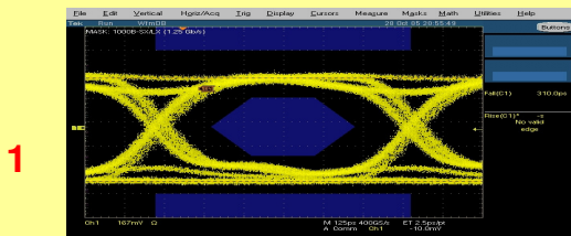
Eye Pattern with Mask: 1000B - SX/LX (1.25Gb/s) at location 1
