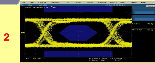
Eye Pattern with Mask: 1000B - SX/LX (1.25Gb/s) at location 2
