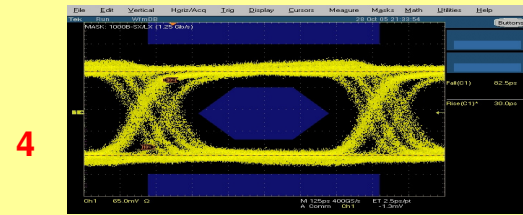
Eye Pattern with Mask: 1000B - SX/LX (1.25Gb/s) at location 4
