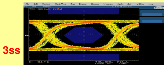
Eye Pattern with Mask: 1000B - SX/LX (1.25Gb/s) at location 3 with single mode Fibre
